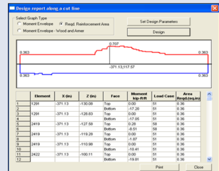
Slab on Grade Design Along any Line
